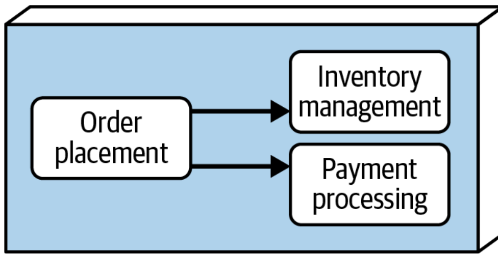
Figure 11-4. Peer-to-peer communication between modules
