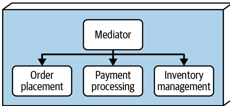
Figure 11-5. The mediator decouples modules, so they don't have to communicate with each other
