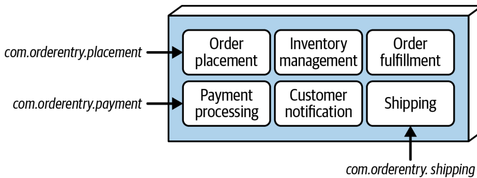
Figure 11-2. An example of the monolithic structure option
